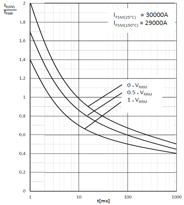
SURGE CHARACTERISTICS
